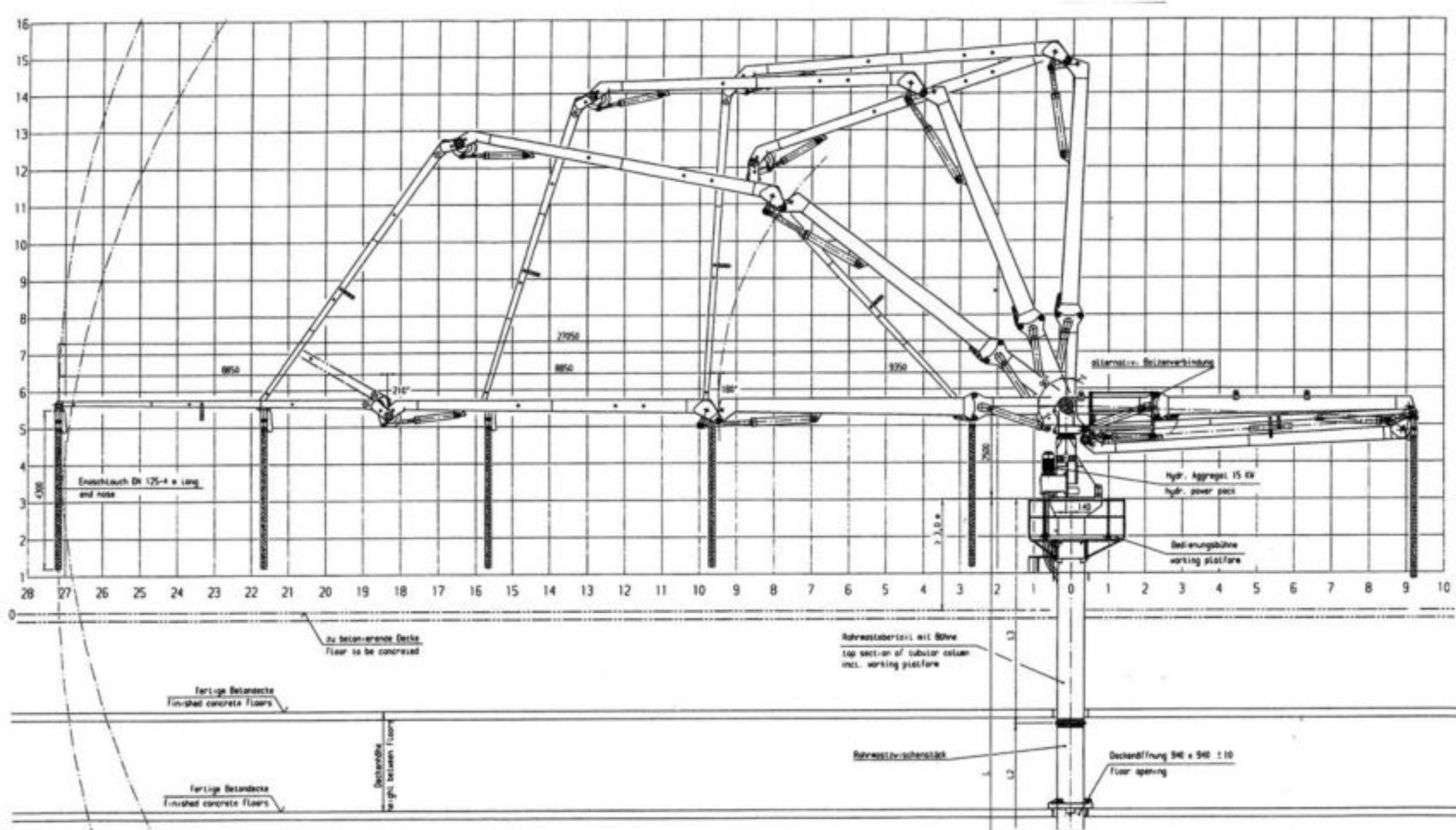
The KVM 27/31 can be mounted on ballasted frames, Cimitec masts, floor held columns or bolted to a base. Maximum free standing is 24 metres with a Cimitec mast, 14 metres with a circular Schwing mast
