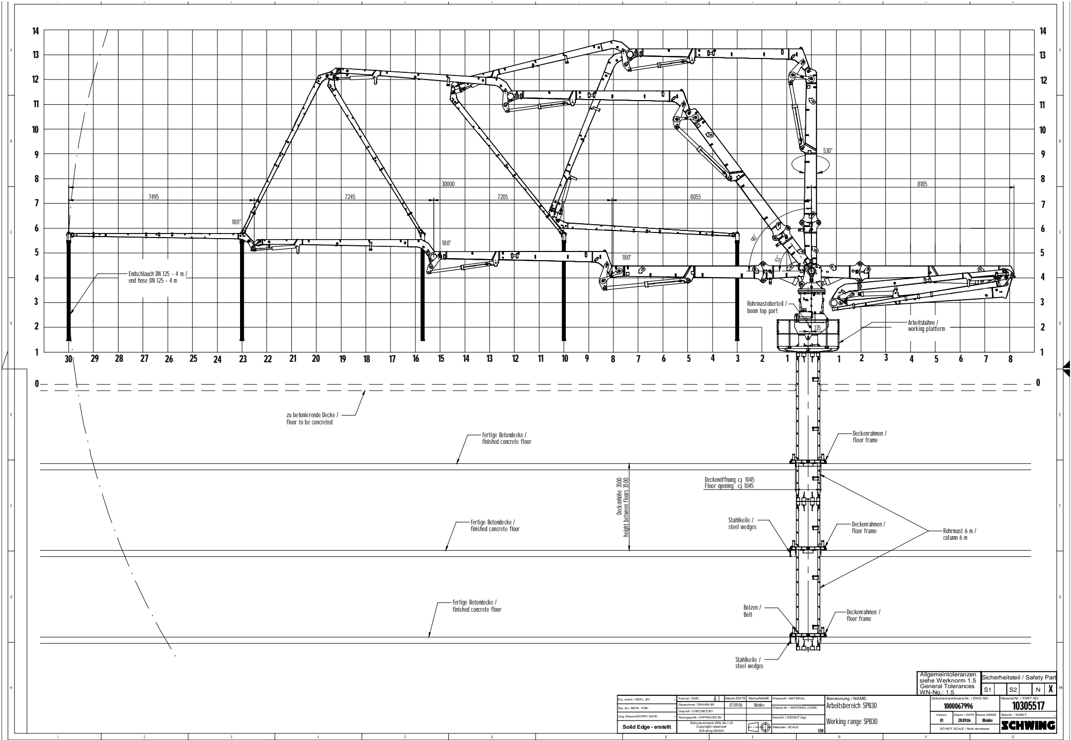
The SPB 30 can be mounted on ballasted frames, self climbing floor held columns or bolted to a base. Maximum free standing is 20 metres with an octagonal Schwing mast
